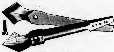
OPEN FOR SHARPENING
